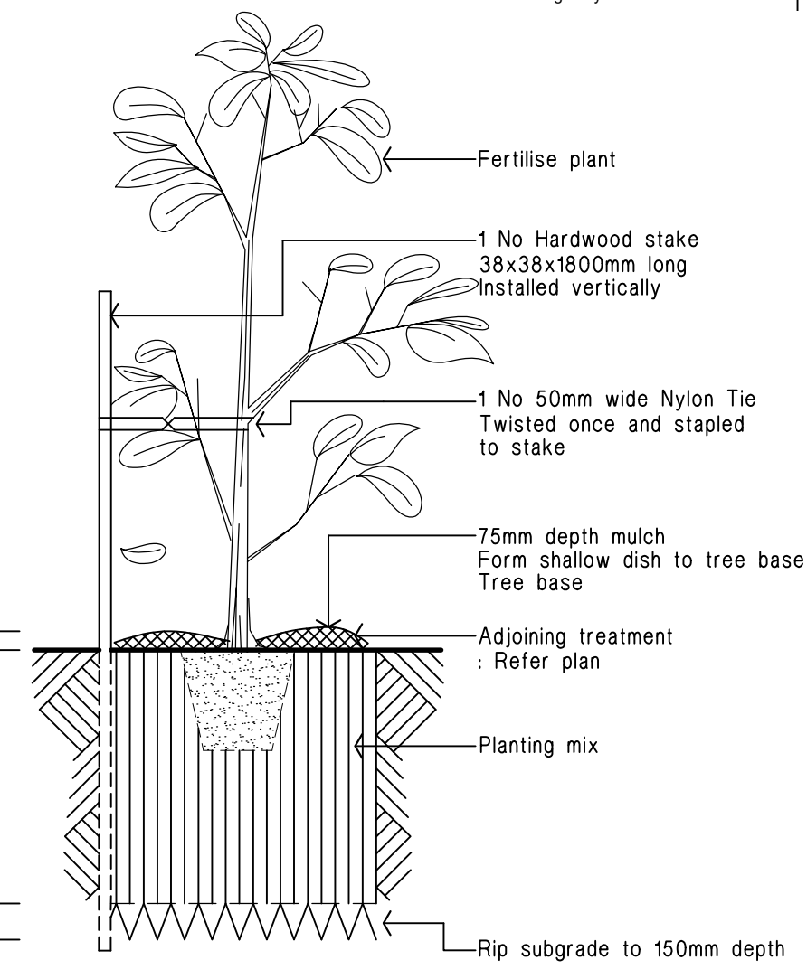
15 - 45 litre Tree planting Detail. Not To Scale.
