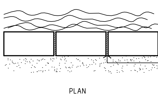
Brick garden edge Detail.
