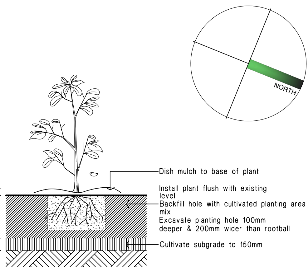
Planting in garden beds Detail. Not To Scale.
